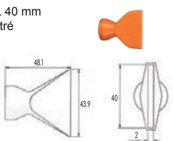
Buse plate L 47.3 mm x Ep. 4.6 mm
