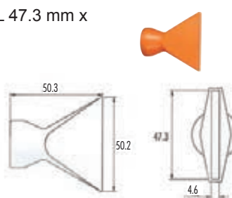
Buse plate L 61 mm x Ep. 3.4 mm
