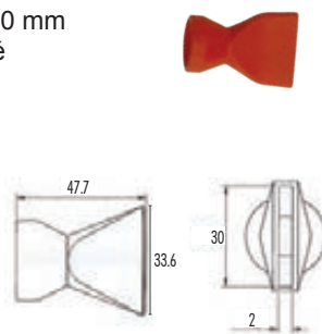
Buse plate L 31.9 mm x Ep. 4.5 mm
